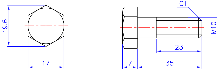
CIMC-D27-02 Door Screw M10X35 螺栓
