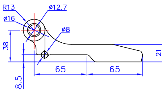
CIMC-D24-04 Maersk Type
