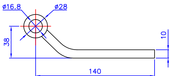
CIMC-D24-03 Welding Type
