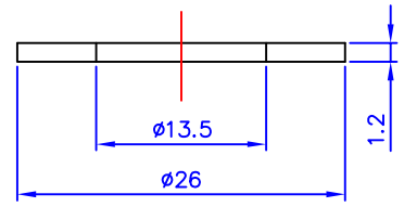
CIMC-D24-07 Brass Wash 铜垫片 Material: Brass
